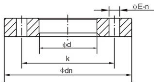
Nylon Coated Flange Plate (PN1.0MPa)
