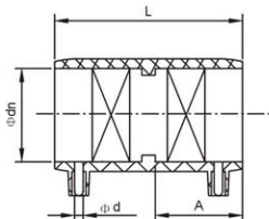
Electrofusion Coupler
