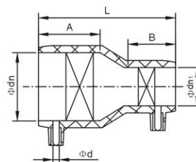
Electrofusion Reducer
