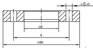
Nylon Coated Flange Plate (PN1.6MPa)
